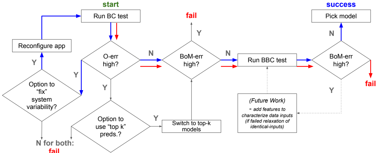
Figure 8: Methodology blueprint. As examples from our findings: Terasort’s path (shown in blue) started out with only 73% of prediction tests having an O-err <10\% in our BC test but once we eliminated its root-cause of irreducible error (the worker-readiness optimization), 99+% of test cases saw an O-err <10\% and the BoM-err even in our BBC test was <10\% for \sim 90\% of test cases leading to what we would deem a successful outcome. By contrast, KMeans (shown by the red path) started with a good O-err in our BC test ( >90\% of test cases had O-err <10\% ) but ultimately failed when we relaxed our identical-inputs assumption where point >60\% of prediction tests had O-err >20\% !
