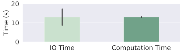
Figure 12: Breakdowns of Spark KMeans job completion time as time spent on cloud storage IO (writing the results to S3) and on computation for 100 experiment runs.
