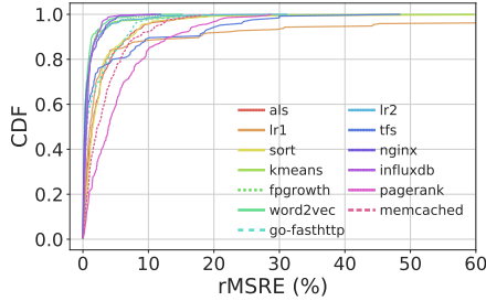
Figure 6: CDF of BoM-err in the BC test where models with prob. outputs are used ( k=3 ). Compare to Fig. 1b.
